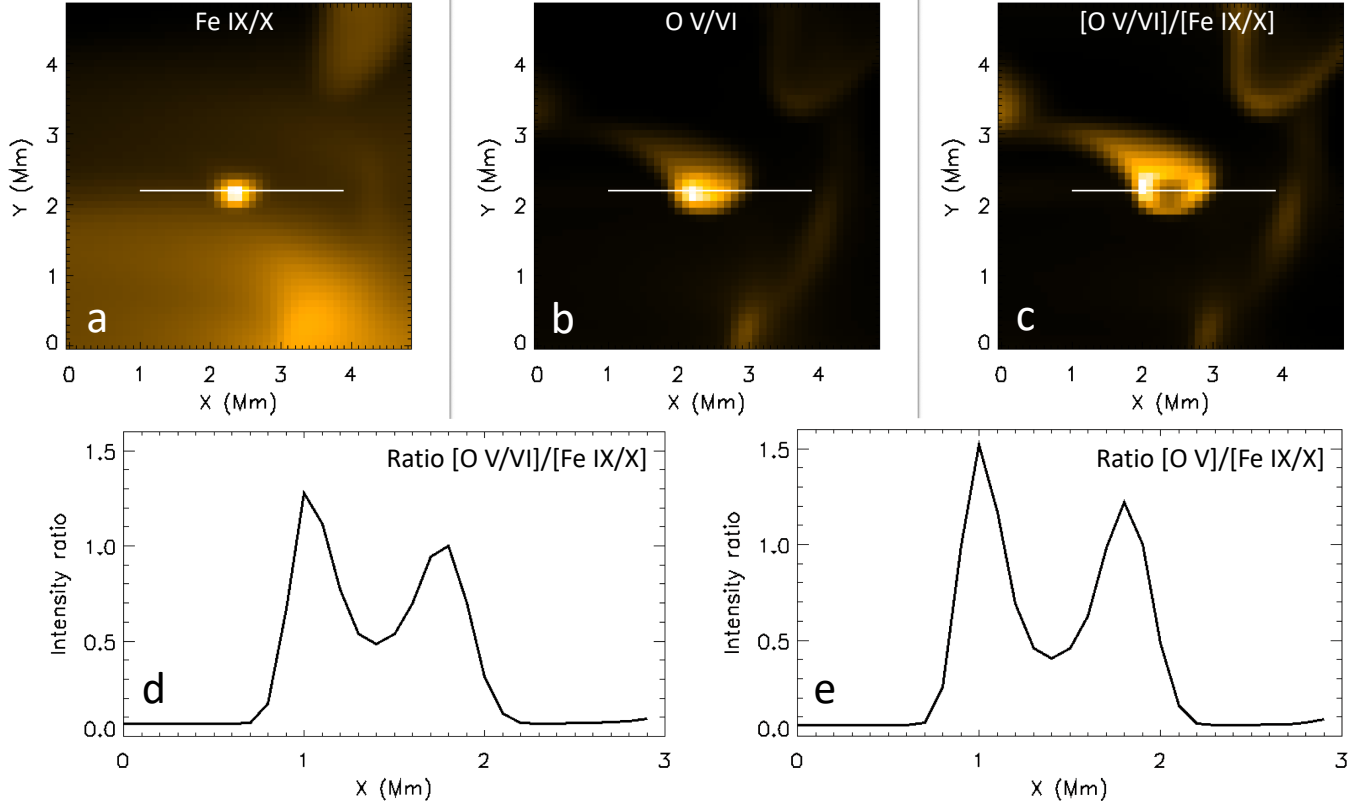
Figure 10. Line ratios of O V/VI to Fe IX/X for a typical dot from the Bifrost MHD simulation. Panels a and b show the images of the dot in Fe IX/X and O V/VI lines. The panel c contains the image of the ratio of O V/VI to Fe IX/X lines. A horizontal line in each panel crosses the dot in the horizontal direction. Panels d and e show the intensity profiles of the ratios [O\ V/VI]/[Fe\ IX/X] and [O\ V]/[Fe\ IX/X] along the horizontal line in panel c. The intensity profiles suggest that the O V/VI lines are equally strong to the Fe IX/X lines and could play a significant role in the appearance of dots observed with HRI EUV .
