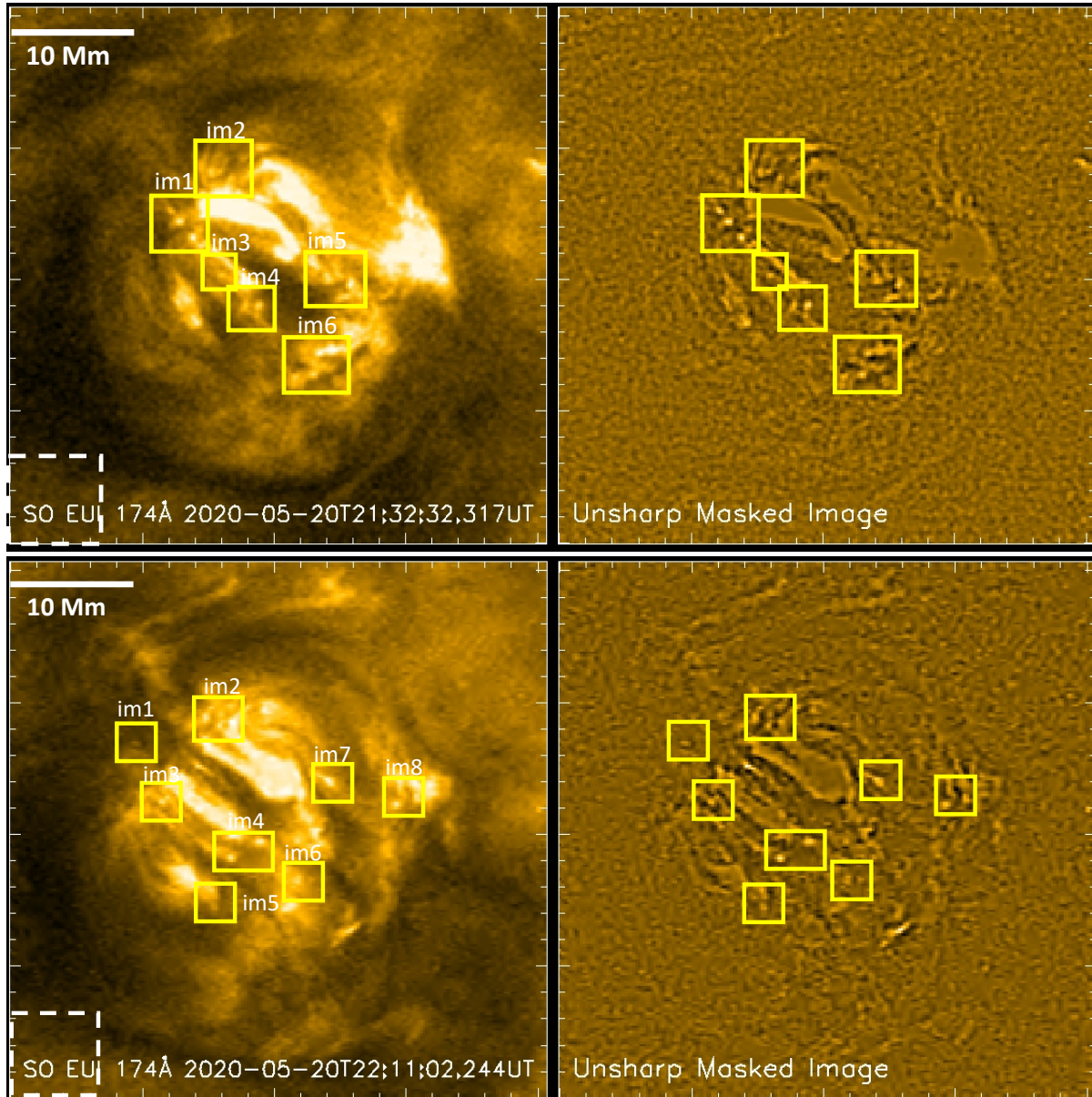
Figure 14. Additional examples of dots in EUV/ \text{HRI}_{\text{EUV}} observations. The left panel in each row is \text{HRI}_{\text{EUV}} 174 Å image, and the right panel is unsharp masked image of it. Different boxes outline the regions of selected dots in each image frame. A white dashed box on the bottom left of the left panel outlines the region that is used for noise estimation. A white horizontal bar on the 174 Å image scales 10 Mm distance, for reference.
